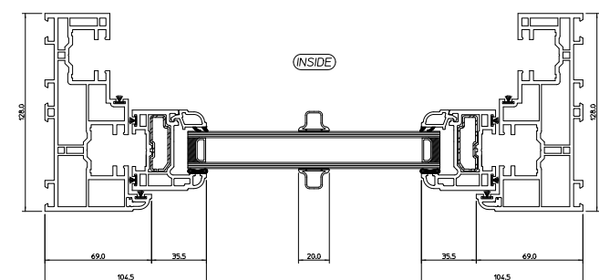
Bottom Sash Downwards View
