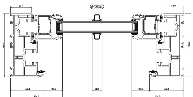
Top Sash Downwards View
