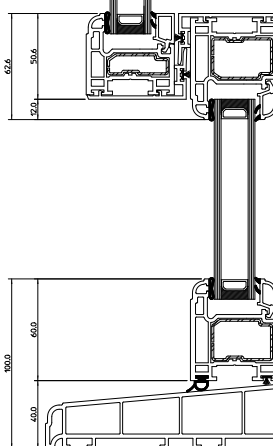
Sideways View - Standard Bottom Rail
